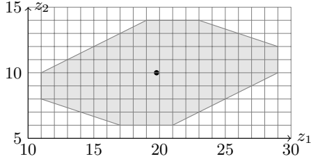
Figure 1: Zonotope \gamma(Z) of Example 3.
