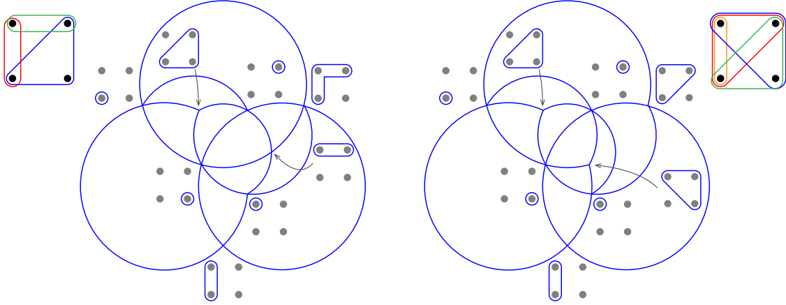
FIGURE 7. Two nested fans. The rays are labeled by the corresponding blocks. As the fans are 3-dimensional, we intersect them with the sphere and stereographically project them from the direction (-1, -1, -1) .
