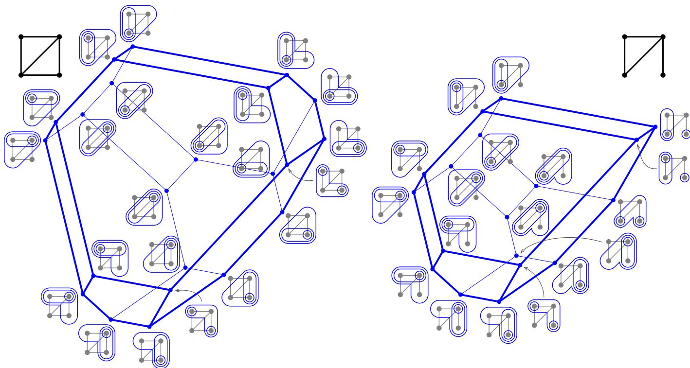
FIGURE 5. Two graph associahedra, realizing the graphical nested fans of Figure 4. The vertices are labeled by the corresponding maximal tubings.
