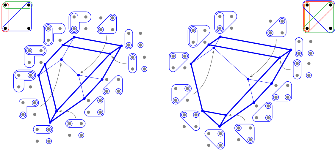
FIGURE 8. Two nestohedra, realizing the nested fans of Figure 7. The vertices are labeled by the corresponding maximal nested sets.
