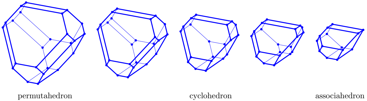
FIGURE 1. A sequence of polytope deformations, from the permutahedron, through the cyclohedron, to the associahedron.
