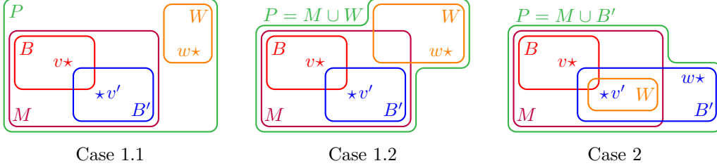
FIGURE 9. Illustrations for the case analysis of the proof of Theorem 3.26.
