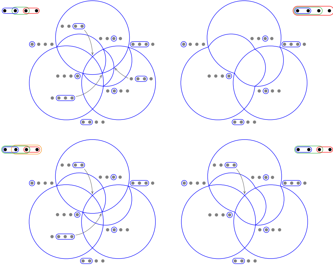
FIGURE 10. Four interval nested fans. The top left one is the Sylvester fan, the top right one is the Pitman-Stanley fan, the bottom left one is the freehedron fan, and only the top right one is a fertilitope fan. The rays are labeled by the corresponding blocks. As the fans are 3-dimensional, we intersect them with the sphere and stereographically project them from the direction (-1, -1, -1) .
