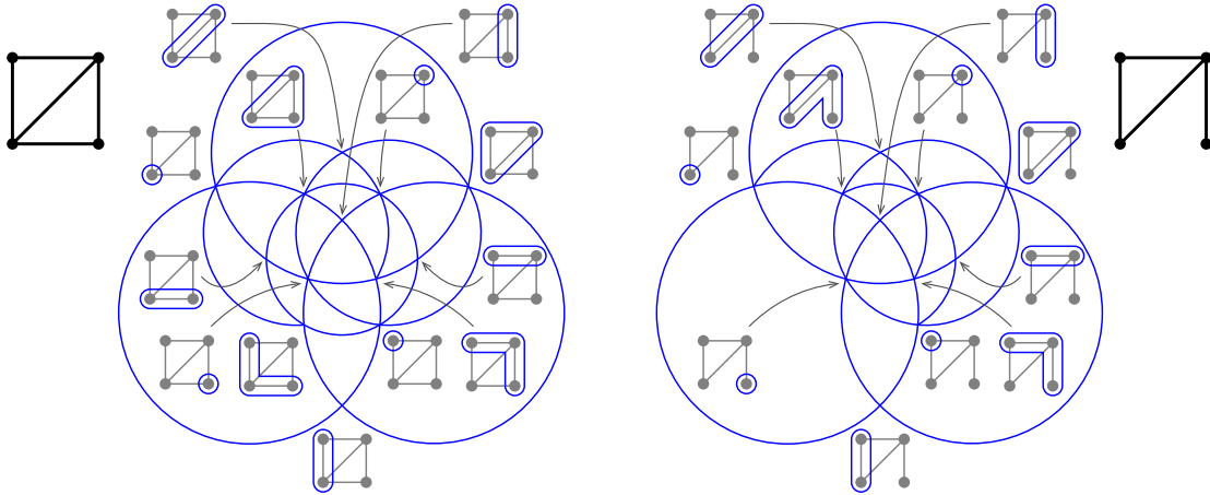
FIGURE 4. Two graphical nested fans. The rays are labeled by the corresponding tubes. As the fans are 3-dimensional, we intersect them with the sphere and stereographically project them from the direction (-1, -1, -1) .
