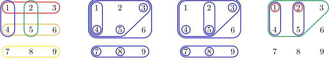
FIGURE 6. The elementary blocks of a building set \mathcal{B}_\circ (left), two adjacent maximal \mathcal{B}_\circ -nested sets (middle), and the corresponding frame (right).
