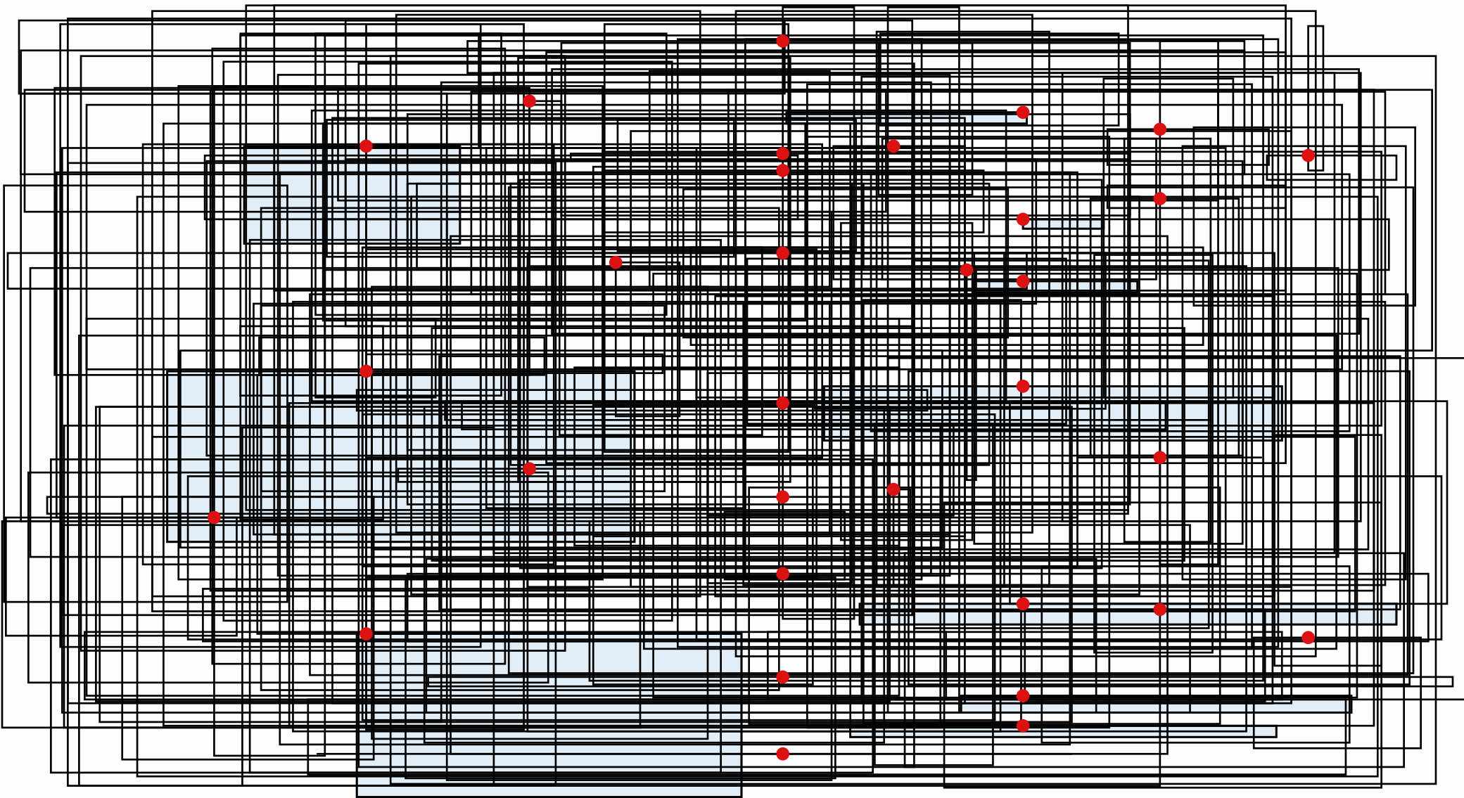
Rectangles : 200 - Stabbing points : 32 - Size of computed pairwise nonintersecting set : 10
