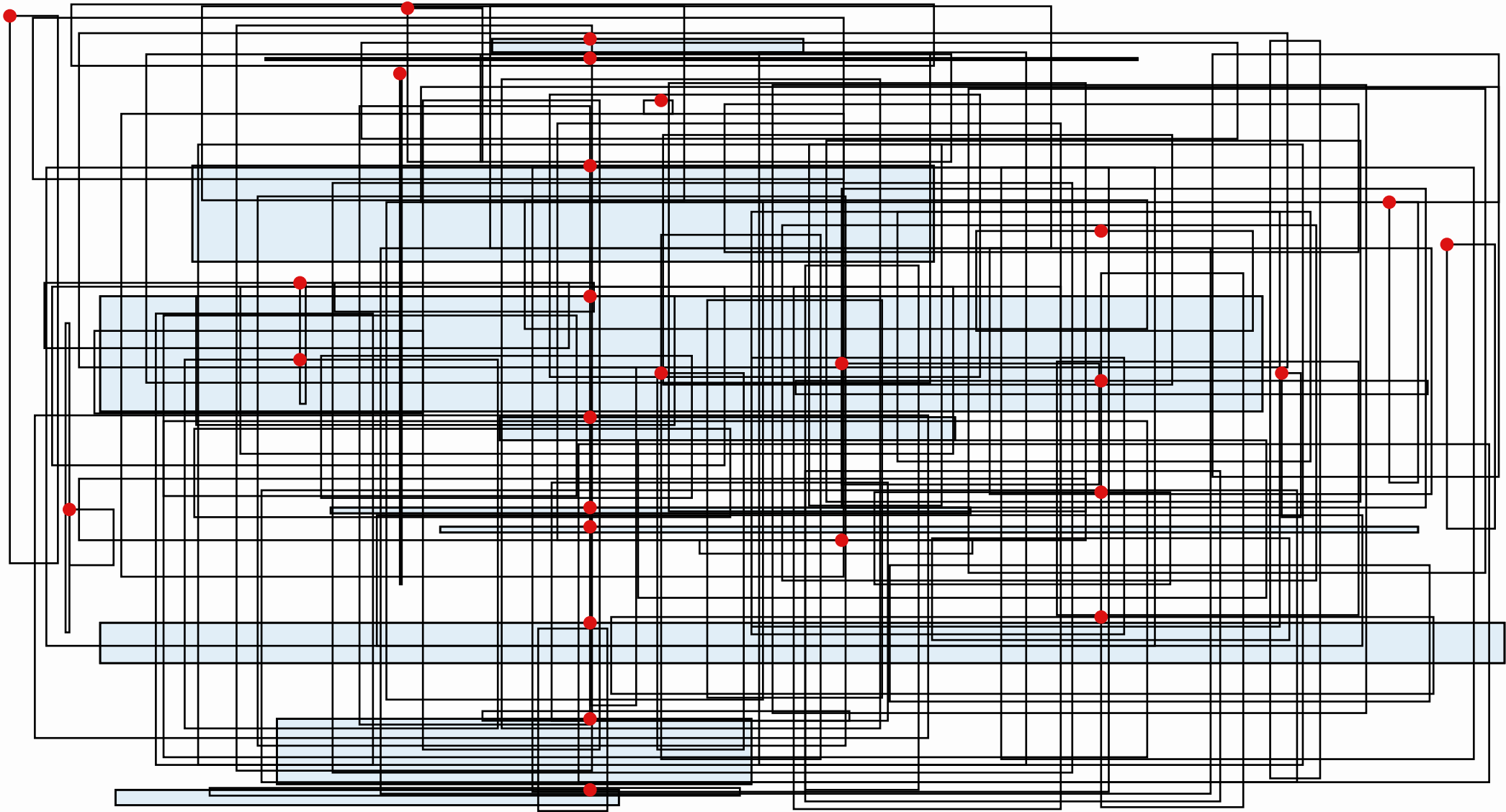
Rectangles : 100 - Stabbing points : 27 - Size of computed pairwise nonintersecting set : 10
