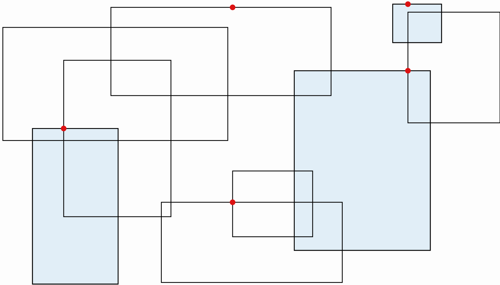
Rectangles : 9 - Stabbing points : 5 - Size of computed pairwise nonintersecting set : 3
