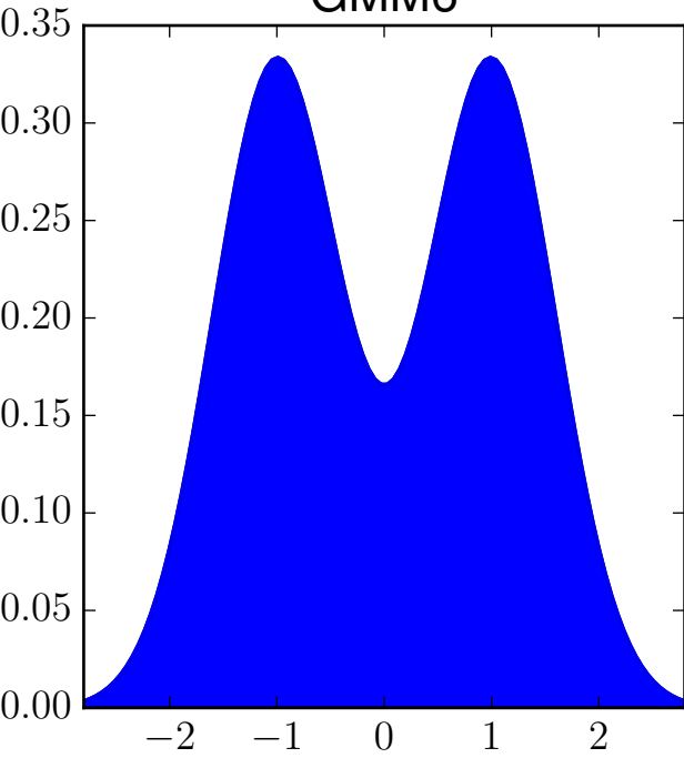
GMM6
