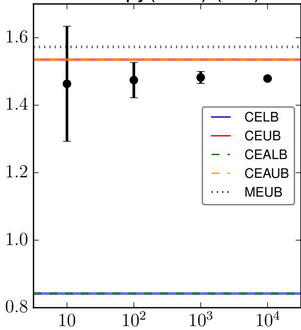
Entropy(GMM6) (0%)
