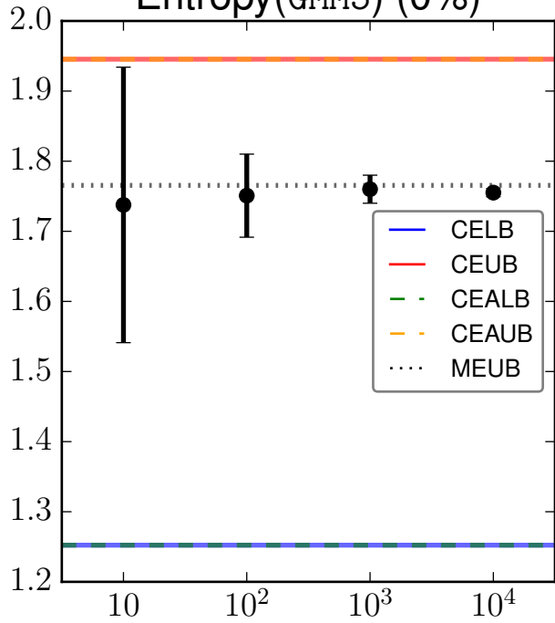
Entropy(GMM5) (0%)
