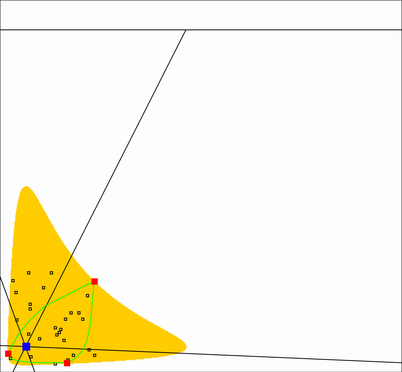
Bregman divergence: Itakura-Saito Divergence (n=30) Center point: (0,255 0,255) – Radius:1,119
