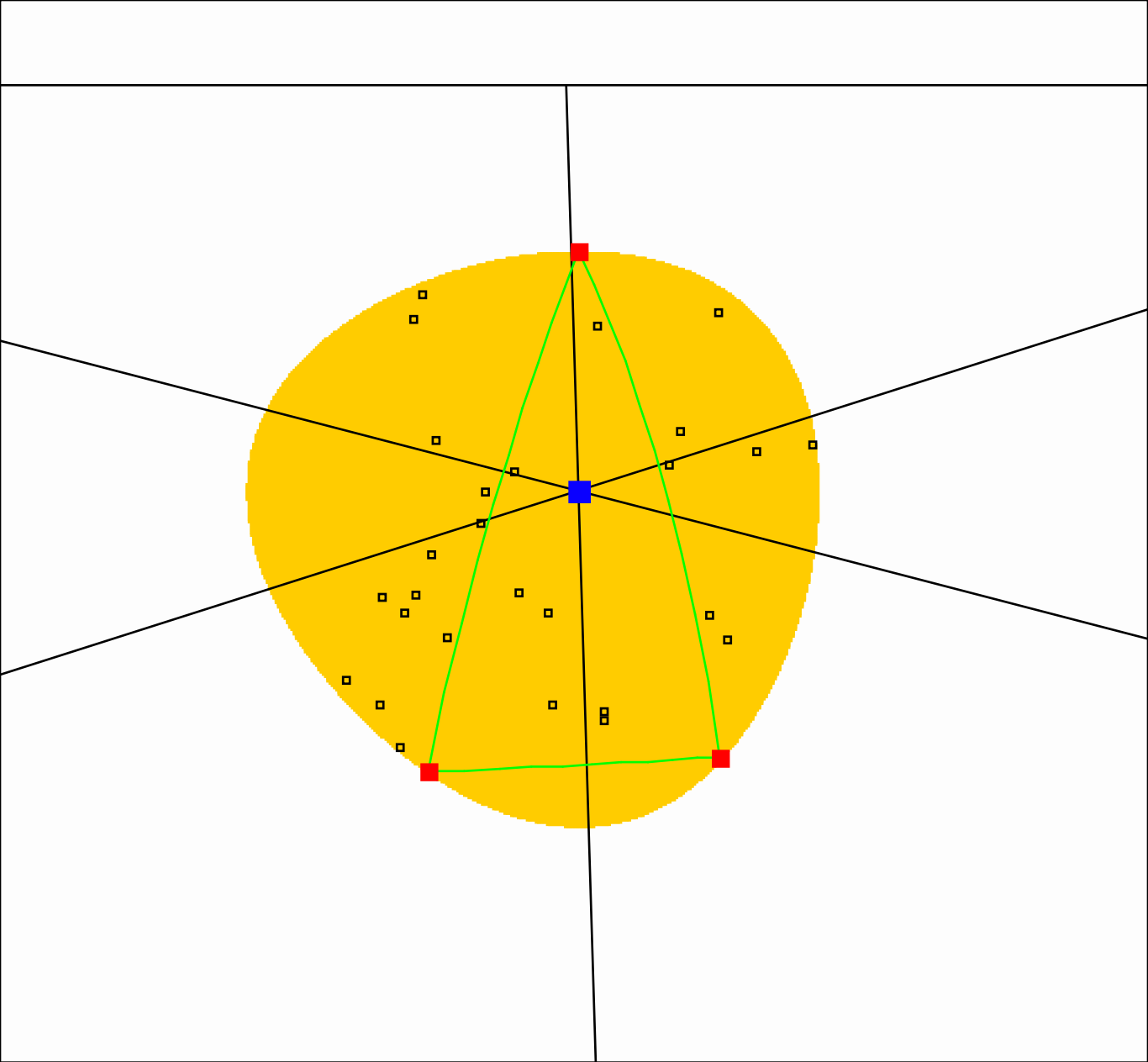
Bregman divergence: Exponential distance (n=30) Center point: (0,508 0,496) – Radius:0,191
