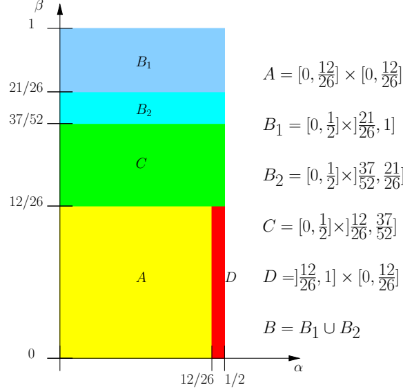
Figure 5: Partition of [0, \frac{1}{2}] \times [0, 1] into five zones.
