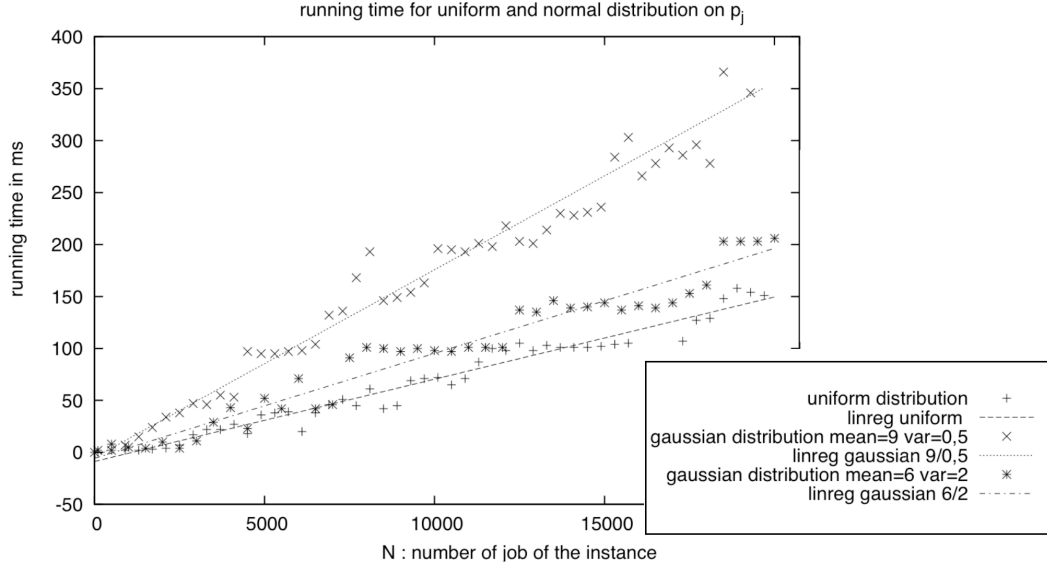
Figure 2: Running time of Algorithm 3.
