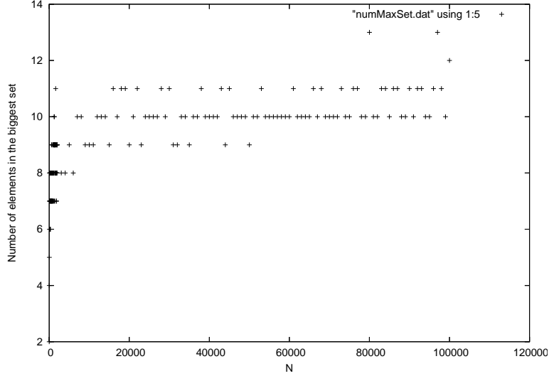
Figure 3: Maximum size of the sets H_j .
