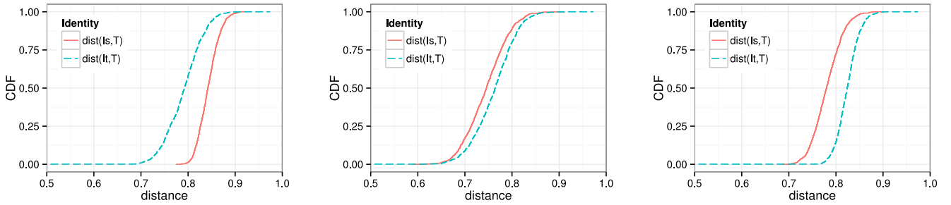
(a) Case of underestimation of the linkability risk (for user id 480480). (b) Case of good estimation of the linkability risk (for user id 535630). (c) Case of overestimation of the linkability risk (for user id 569318).
