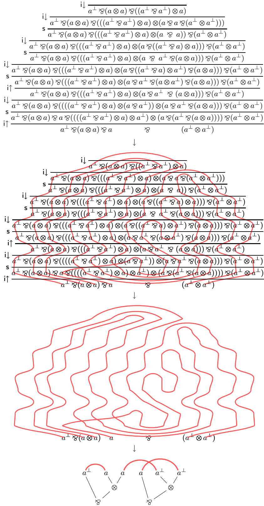
Figure 7: From calculus of structures to proof nets
