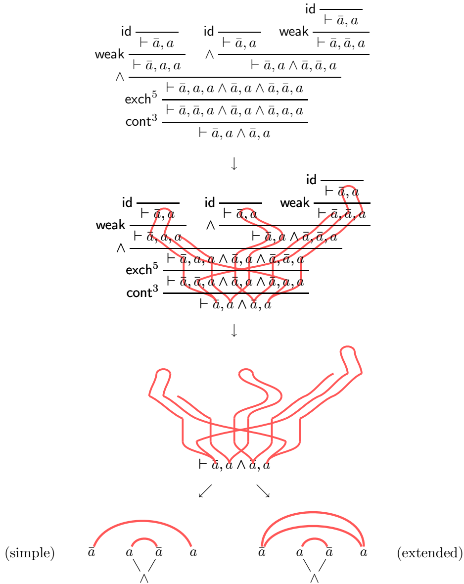
Figure 16: From sequent calculus to classical logic proof nets via flow graphs
