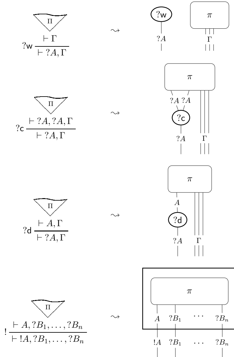
Figure 10: From sequent calculus to proof nets: exponentials
