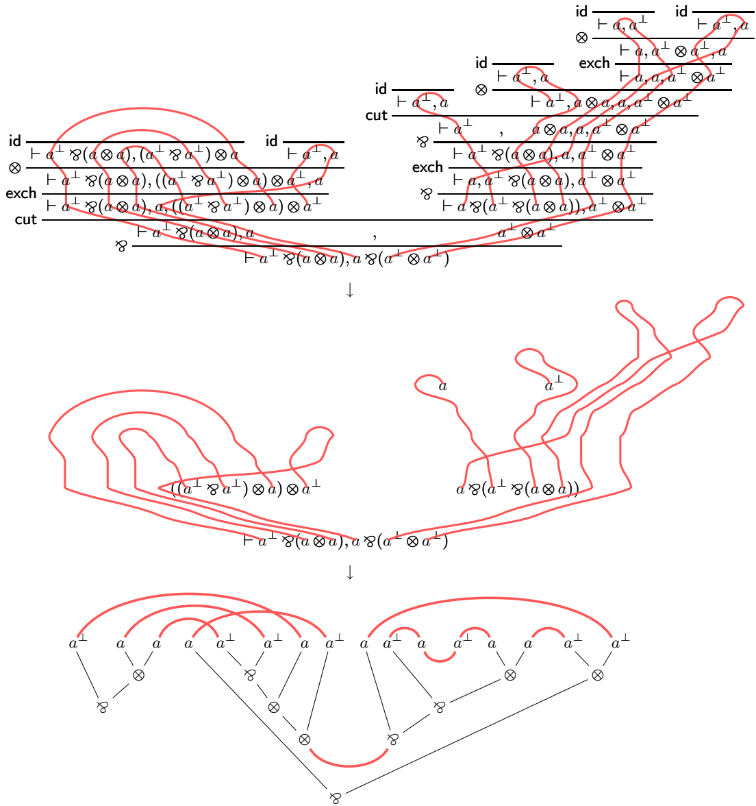
Figure 4: From sequent calculus to proof nets with cuts via coherence graphs
