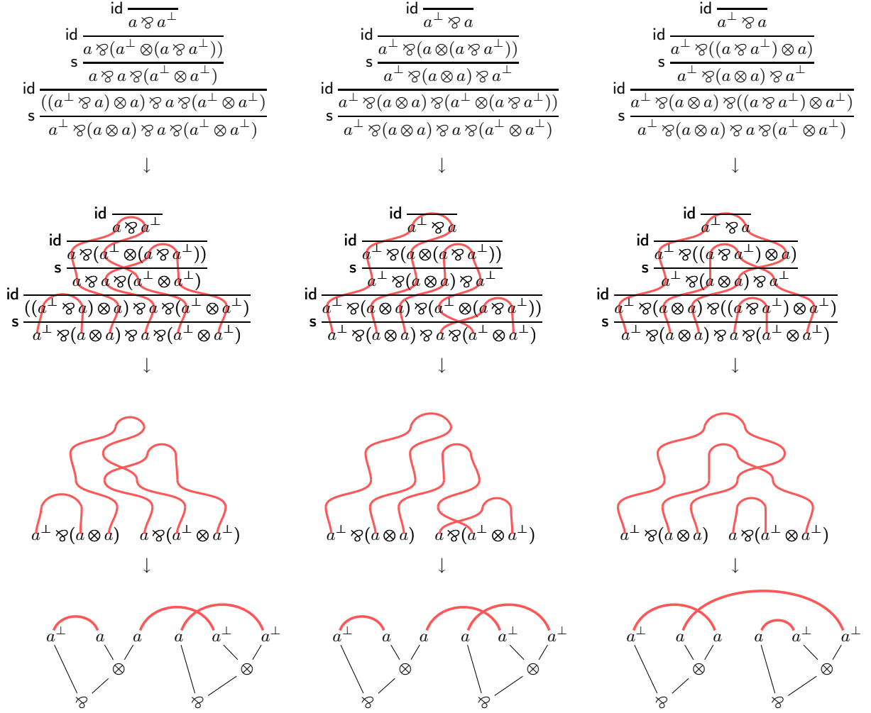
Figure 6: From calculus of structures to proof nets
