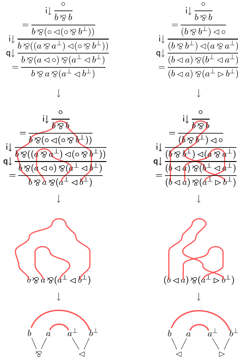
Figure 15: From BV to proof nets
