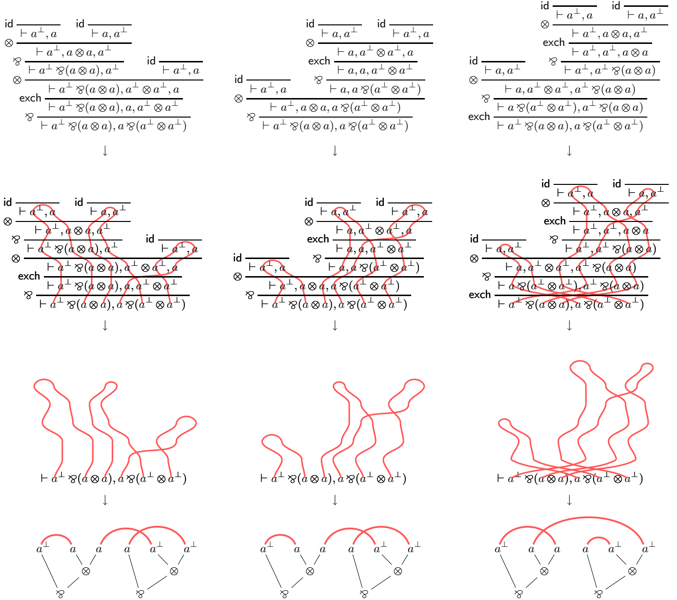
Figure 2: From sequent calculus to proof nets via coherence graphs
