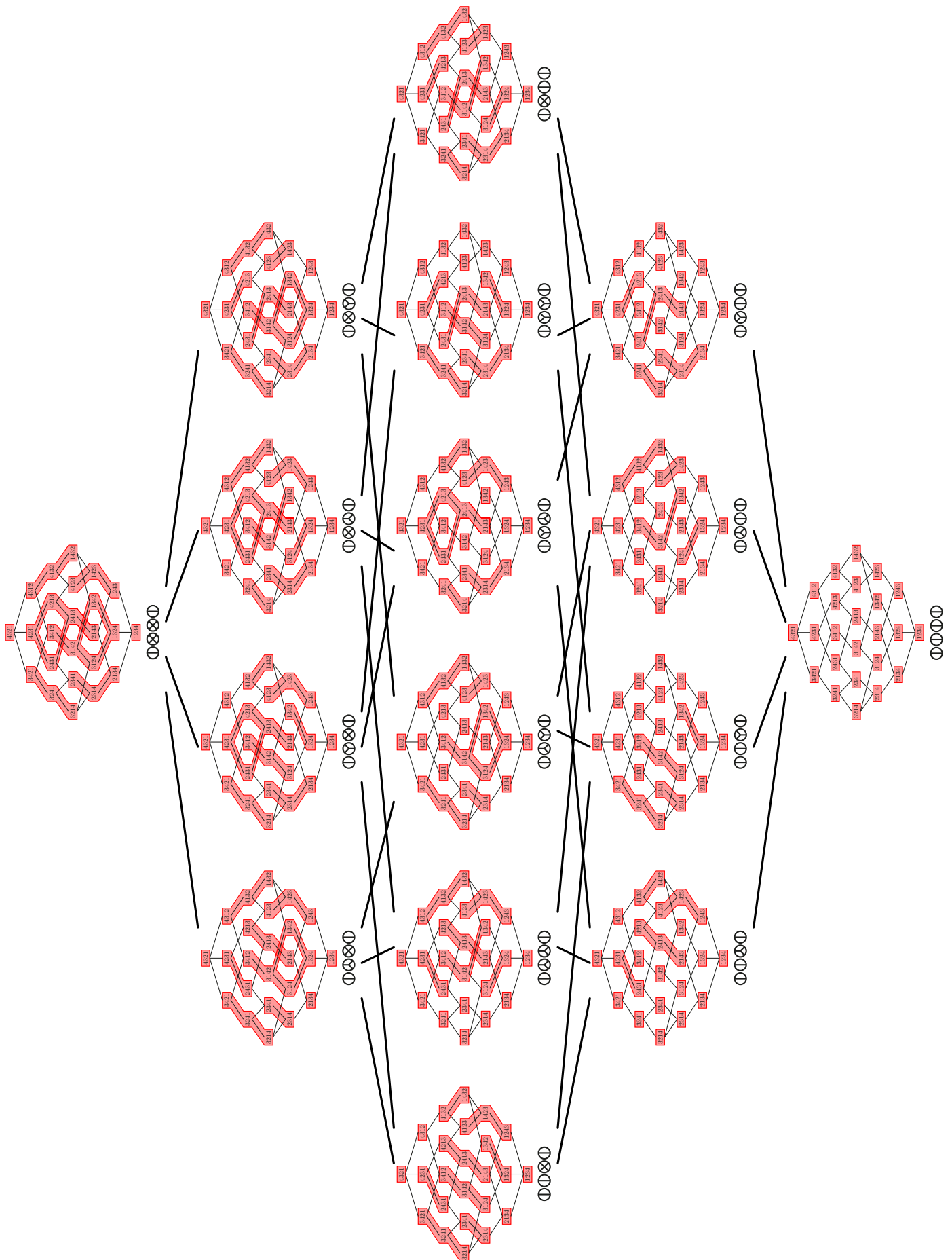
FIGURE 13. The fibers of the \delta -permutree congruence, for all decorations \delta \in \mathbb{O} \cdot \{\mathbb{O}, \otimes, \ominus, \otimes, \otimes\}^2 \cdot \mathbb{O} .
