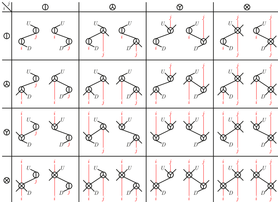
FIGURE 8. Rotations in permutrees: in each box, the tree T (left) is transformed into the tree T' (right) by rotation of the edge i \rightarrow j . The 16 boxes correspond to the possible decorations of i and j .
