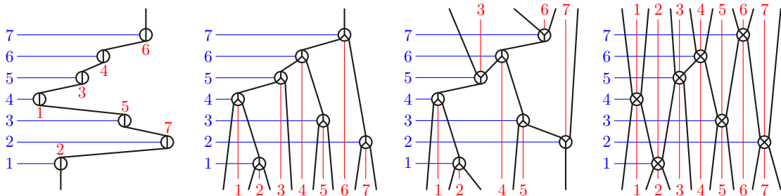
FIGURE 2. Leveled permutrees corresponding to a permutation (left), a leveled binary tree (middle left), a leveled Cambrian tree (middle right), and a leveled binary sequence (right).
