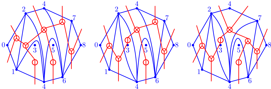
FIGURE 9. A sequence of two rotations on permutrees, and the corresponding flips on \{2, 3, 4\} -angulations.
