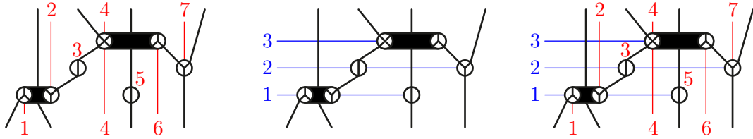
FIGURE 20. A Schröder permutree (left), an increasing tree (middle), and a 3-leveled Schröder permutree (right).
