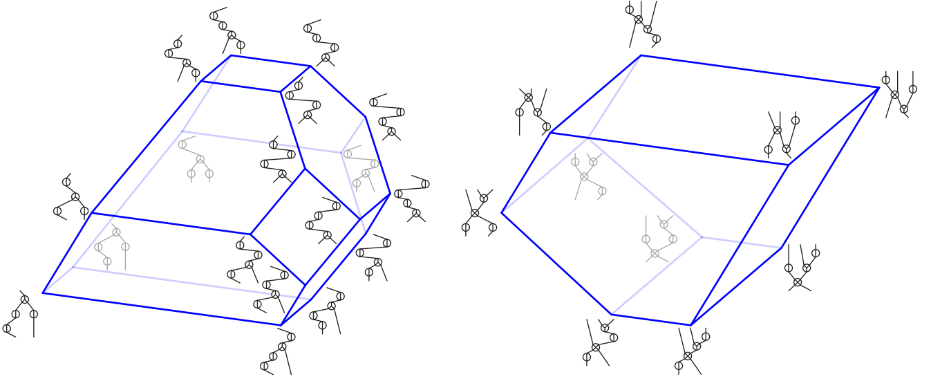
FIGURE 14. The permutreehedra \text{PT}(\odot\odot\otimes\odot) (left) and \text{PT}(\odot\otimes\otimes\odot) (right).
