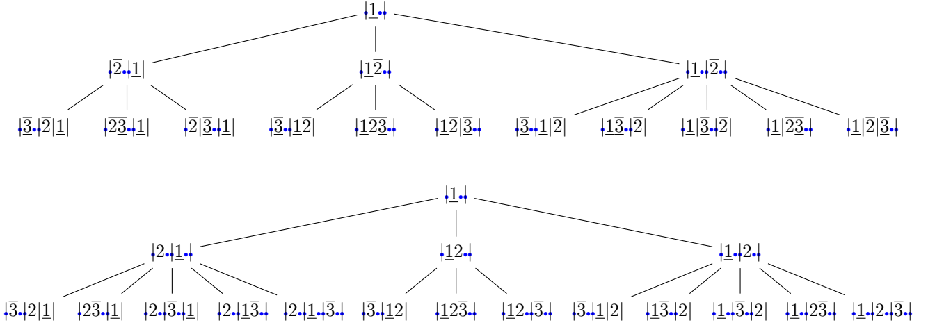
FIGURE 25. The generating trees \mathcal{S}_\delta for the decorations \delta = \textcircled{\times} (top) and \delta = \textcircled{\cdot} (bottom). Free gaps are marked with a blue dot.
