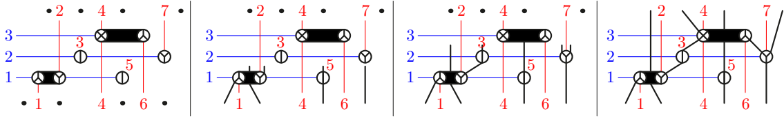
FIGURE 23. The insertion algorithm on the signed ordered partition \underline{125|37|46} .
