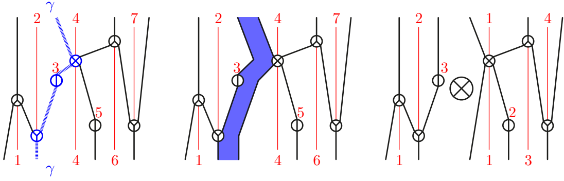
FIGURE 18. A gap \gamma between 2 and 3 (left) defines a vertical cut (middle) which splits the permutree vertically (right).
