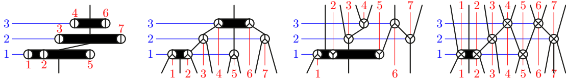
FIGURE 21. Leveled Schröder permutrees corresponding to an ordered partition (left), a leveled Schröder tree (middle left), a leveled Schröder Cambrian tree (middle right), and a leveled ternary sequence (right).
