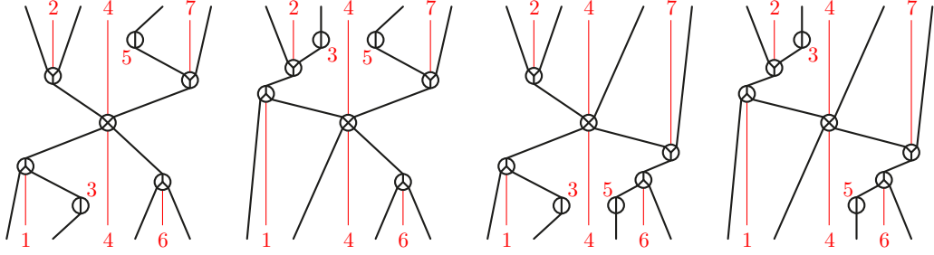
FIGURE 19. The four generators of the upper ideal of \mathbb{E} -indecomposable \delta -permutrees for the decoration \delta = \textcircled{\ominus}\textcircled{\ominus}\textcircled{\otimes}\textcircled{\ominus}\textcircled{\otimes}\textcircled{\ominus} .
