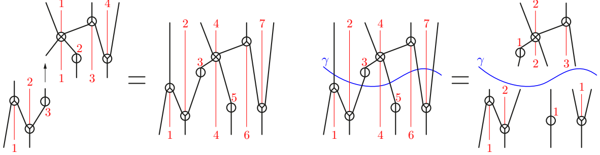
FIGURE 16. Grafting two permutrees (left) and cutting a permutree (right).
