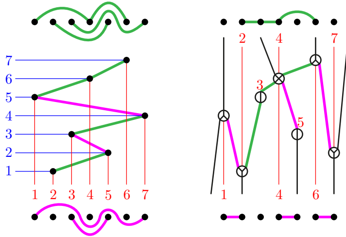
FIGURE 6. The arc diagrams \text{asc}(\tau) (green, up) and \text{desc}(\tau) (pink, down) associated to the permutation \tau = 2537146 (left) and the arc diagrams \text{asc}(T) (green, up) and \text{desc}(T) (pink, down) associated to a permutree T (right).
