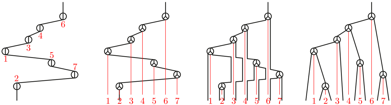
FIGURE 12. BST insertion seen as the refinement map from a \mathbb{D}^n -permutree (i.e. a permutation of \mathfrak{S}_n ) to a \oplus^n -permutree (i.e. a binary tree on [n] ).
