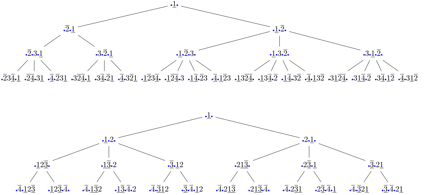
FIGURE 7. The generating trees \mathcal{T}_\delta for the decorations \delta = \textcircled{2}\textcircled{3}\textcircled{4}\textcircled{1} (top) and \delta = \textcircled{1}\textcircled{2}\textcircled{3}\textcircled{4} (bottom). Free gaps are marked with a blue dot.
