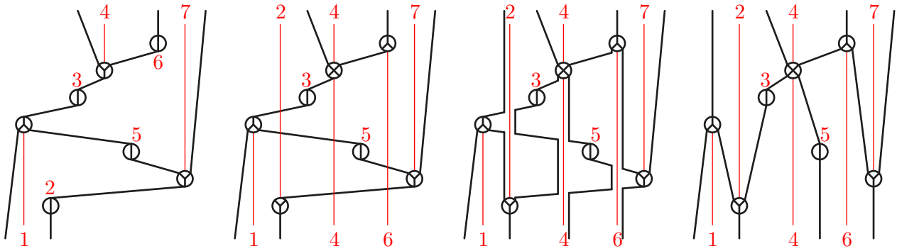
FIGURE 11. Refinement by cut and stretch: starting from a permutree decorated with \oplus\odot\odot\odot\odot\odot\odot (left), we redecorate its vertices with \oplus\odot\odot\otimes\odot\odot\odot (middle left), cut and reconnect its edges along the resulting red walls (middle right), and stretch the resulting \oplus\odot\odot\otimes\odot\odot\odot -permutree (right).
