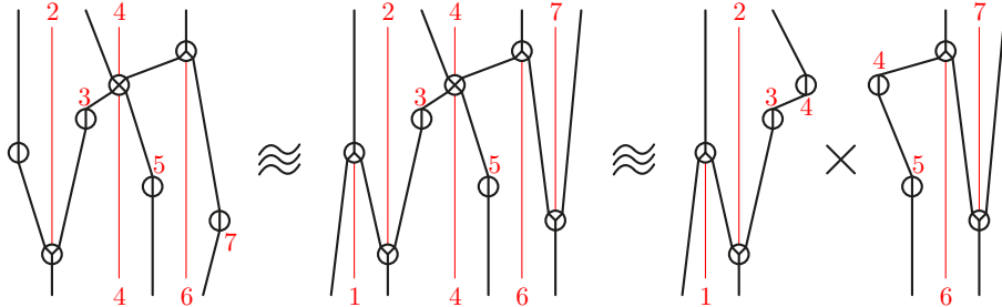
FIGURE 3. Some bijections between permutrees: the leftmost and rightmost decorations do not matter (left), and a decoration \otimes yields a product (right).
