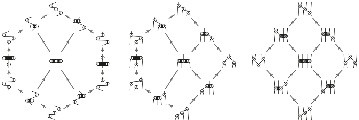
FIGURE 24. The Schröder \delta -permutree lattices for \delta = \circlearrowleft^3 (left), \circlearrowright^3 (middle) and \otimes^3 (right).
