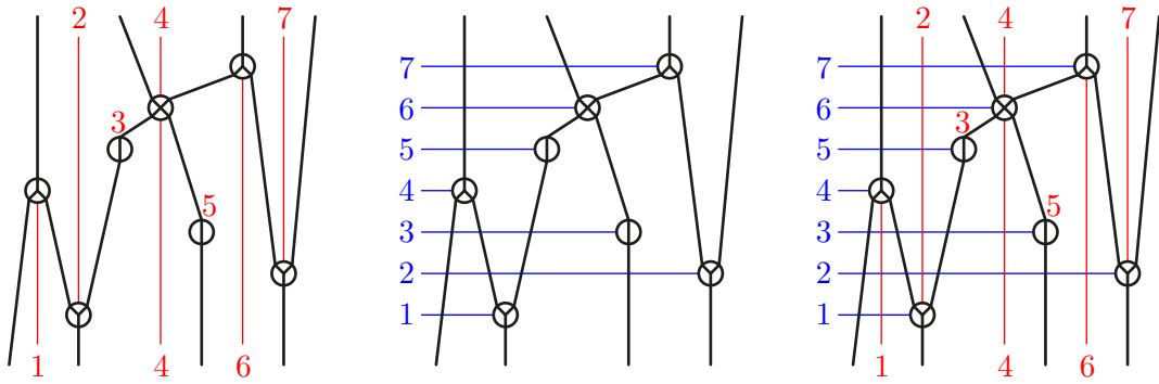
FIGURE 1. A permutree (left), an increasing tree (middle), and a leveled permutree (right). The decoration is \otimes\ominus\oplus\otimes\oplus\otimes\oplus .
