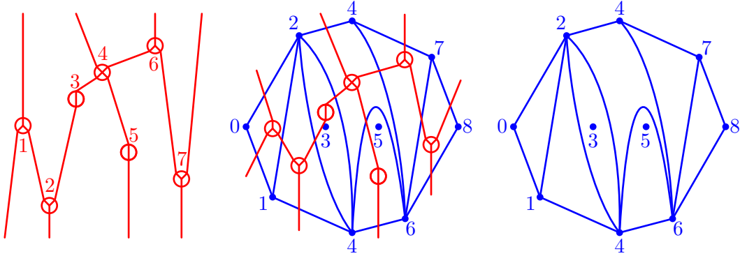
FIGURE 4. Permutrees (left) and \{2, 3, 4\} -angulations (right) are dual to each other.
