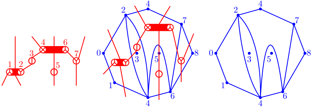
FIGURE 22. Schröder permutrees (left) and dissections (right) are dual to each other.
