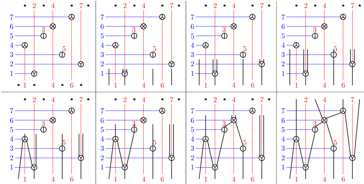
FIGURE 5. The insertion algorithm on the decorated permutation \overline{2751346} .
