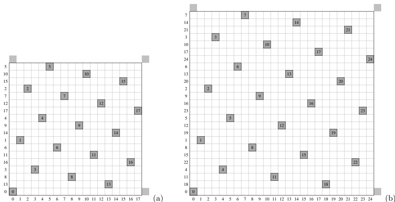
Figure 4: Examples of two optimal families of rook lattices in the square. (a) Lattice generated by the vectors (m, m) and (1, 2m + 1) , for m = 3 . (b) Lattice generated by the vectors (m + 1, m) and (1, 2m + 1) , for m = 3 .
