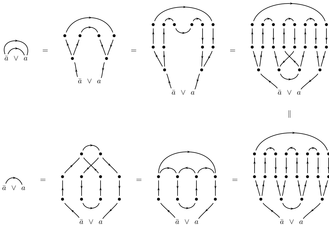
Figure 1: The idea of the proof of Theorem 8.6
