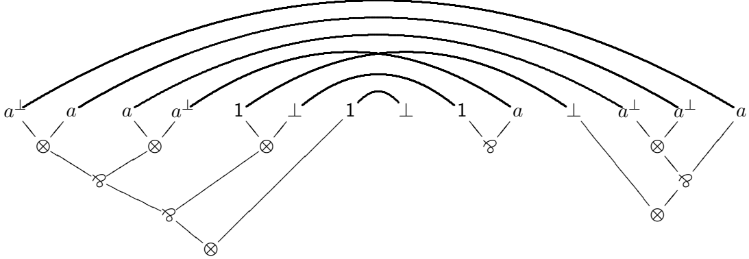
Figure 5: Example of an ordinary proof net
