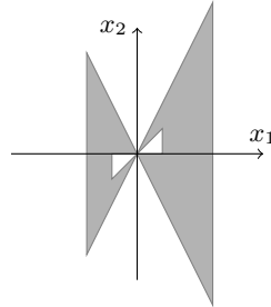
Fig. 6. Evaluation of a non-linear expression \llbracket x_2 \leftarrow x_1 \times x_2 \rrbracket_{1 \setminus 2}^\#
