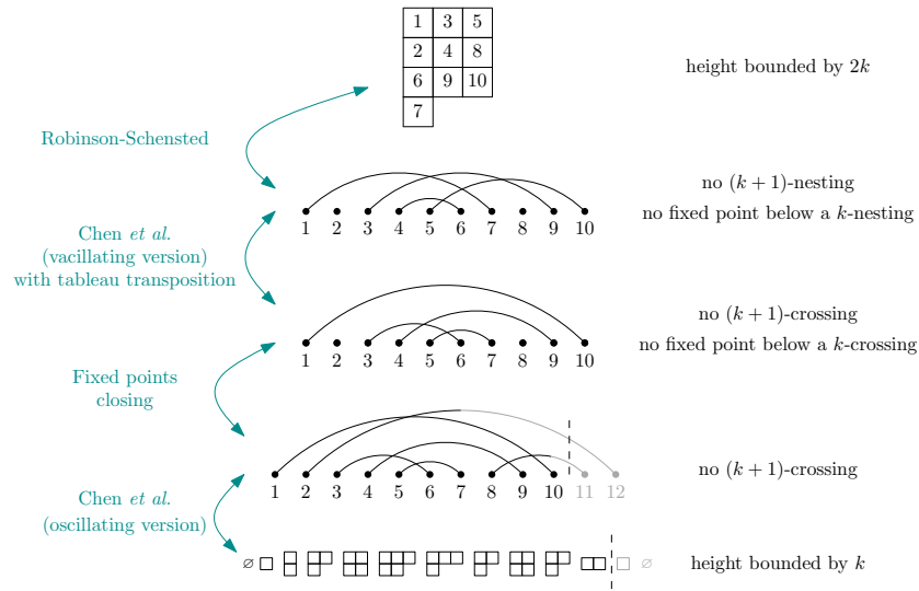
Figure 1: The bijection behind Theorem 1. From top to bottom: standard Young tableau of size n with height bounded by k and m odd columns; involution diagram of size n with m fixed points and no enhanced (k+1) -nesting; involution diagram of size n with m fixed points, and no (k+1) -crossing, nor fixed point below a k -crossing; matching diagram of size n+m with no (k+1) -crossing whose m last arcs are part of an m -nesting; oscillating tableau of size n+m with height bounded by k , whose n th diagram is a row of length m . For this particular example, n = 10 and k = m = 2 .
