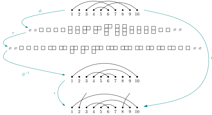
Figure 10: Image of the involution (1\ 7)(3\ 9)(4\ 6)(5\ 10) under \psi .
