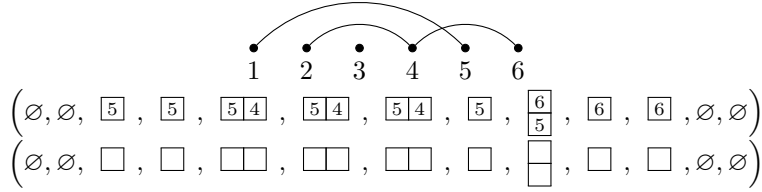
Figure 8: Top. The set partition \pi = \{1, 5\}, \{2, 4, 6\}, \{3\} . Middle. The corresponding Young tableau sequence. Bottom. The vacillating tableau given by \phi(\pi) .
