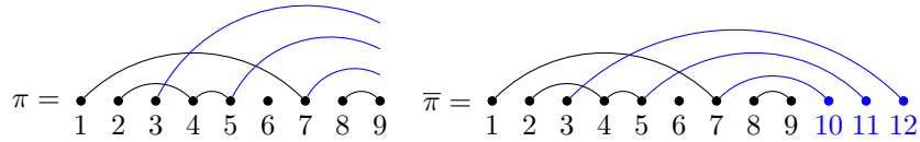
Figure 9: Left. An open partition diagram, \pi , with 3 open arcs. Right. The corresponding closed partition diagram \bar{\pi} ending with a 3-nesting, obtained by closing the 3 open arcs of \pi in reverse order.
