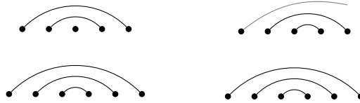
Figure 11: Left. An enhanced 3-nesting with respectively 5 and 6 dots. Right. A 3-nesting with respectively 5 and 6 dots (in an open matching).
