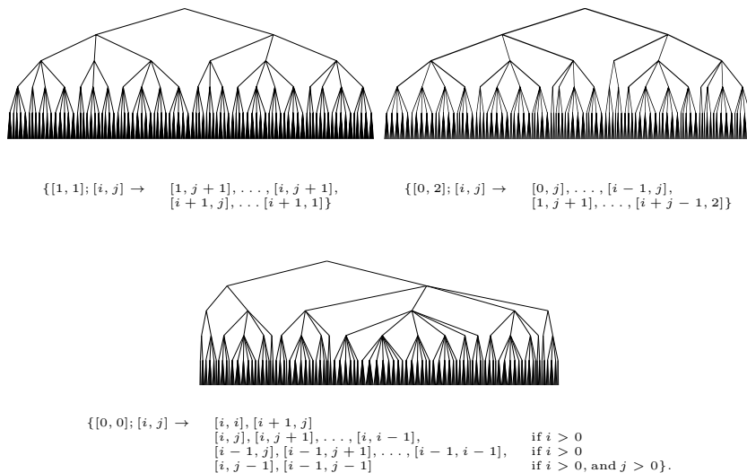
Figure 13: The first five levels of each of the Baxter generating trees. They are respectively from [7] [10] [12].
