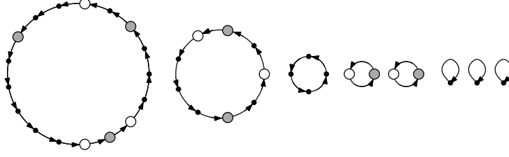
Figure 12: Schematic representation of typical orbits under \theta . The white circles represent the elements of A_{2k,2k+1} , the gray circles the elements of A_{2k+1,2k} and the small points are the remaining elements.
