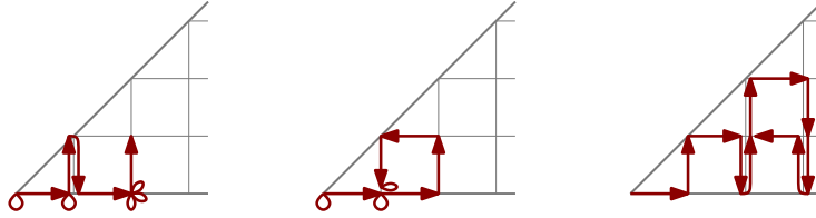
Figure 3: From left to right: a W_2 -vacillating walk; a W_2 -hesitating walk; a W_2 -oscillating walk. The stay steps are drawn as loops. (These walks correspond to the tableaux of FIGURE 2.)
