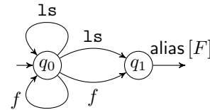
Fig. 8. \mathcal{A}[1s(E, F)]
