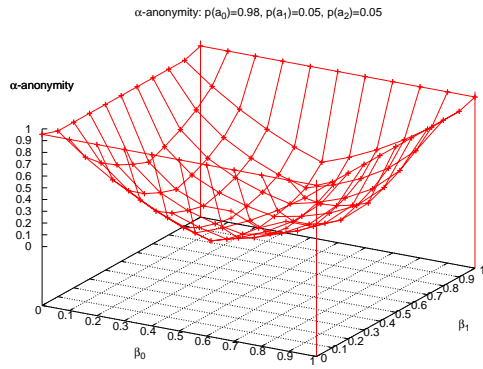
Fig. 6. The dependency of \alpha -anonymity on the \beta_i 's in the case of three cryptographers.
