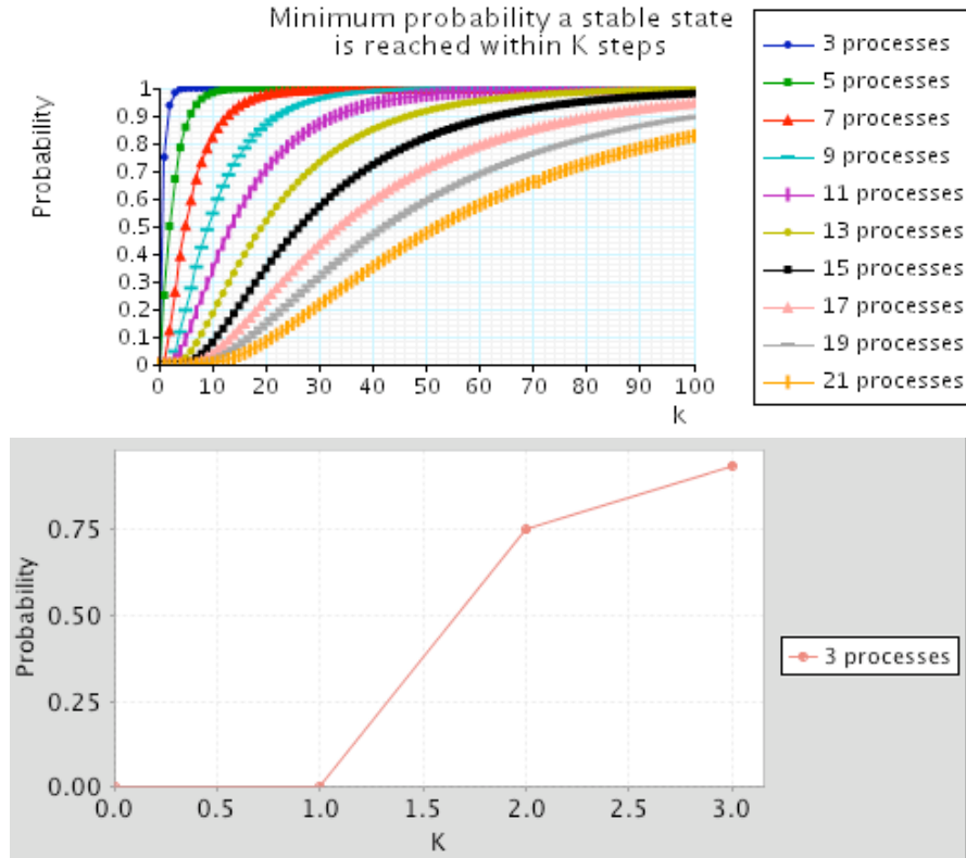
Figure 2: The minimum probability of reaching a stable configuration within K steps
