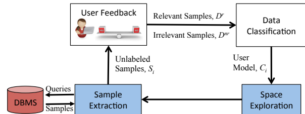
Figure 1: The AIDE framework
