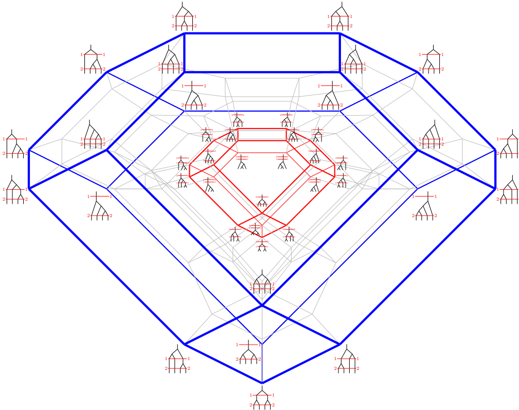
FIGURE 1. The (2, 3) -multiplihedron.
