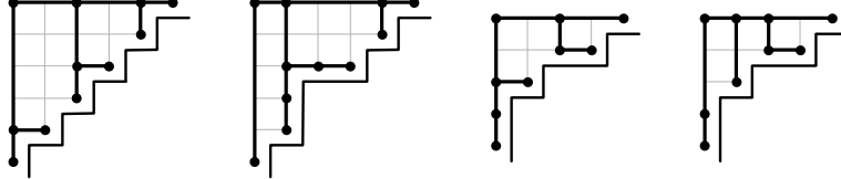
FIGURE 17. Some \nu -trees for different Dyck paths \nu : the first is just the binary tree of Figure 11, the last two are related by a rotation.
