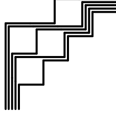
FIGURE 28. The maximal chain \boldsymbol{\pi} .
