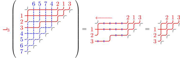
FIGURE 2. Horizontal packing of a pipe dream at k = 3 .
