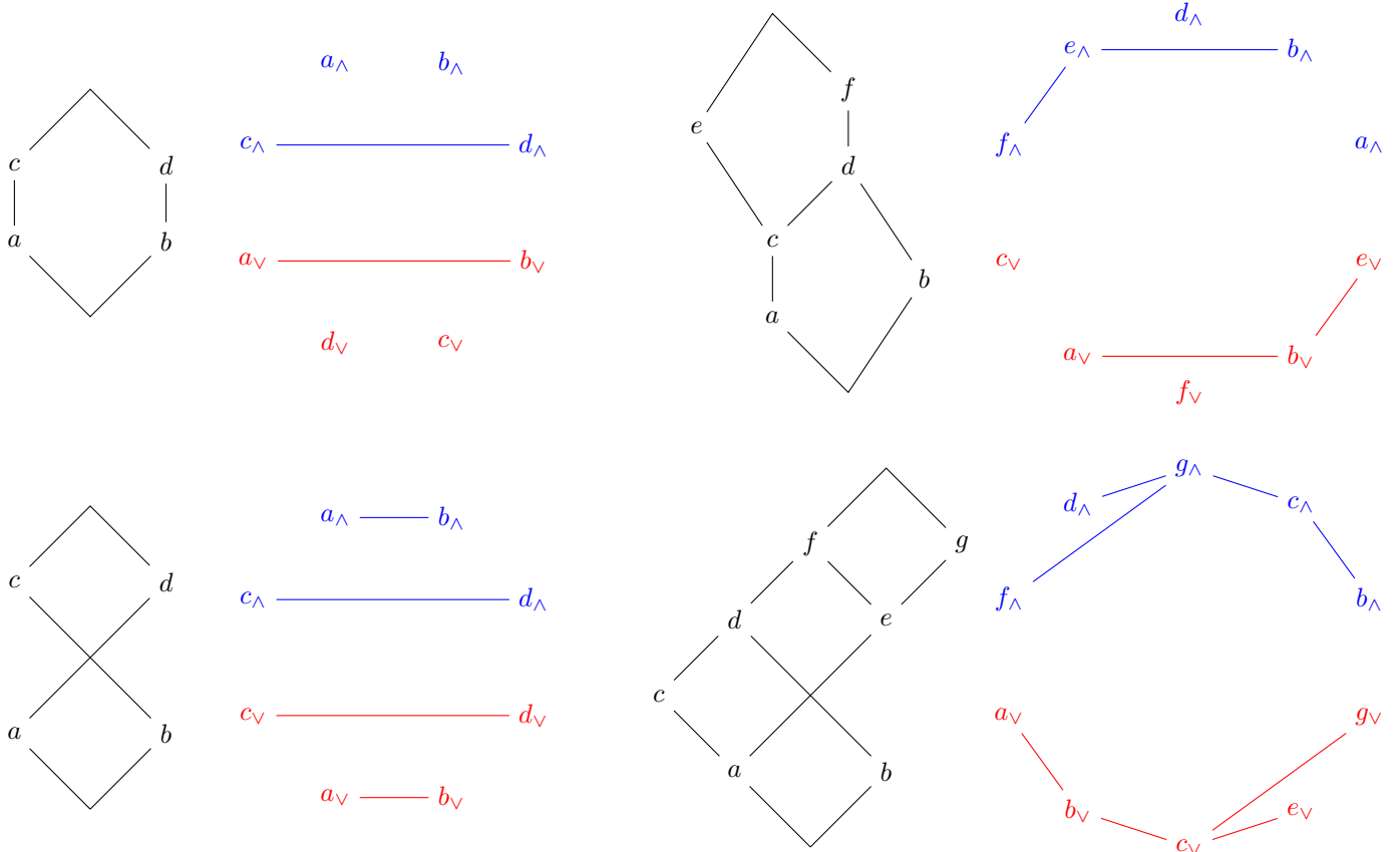
FIGURE 2. Some semidistributive lattices and their canonical join (red) and meet (blue) complexes. The letters label all join or meet irreducible elements, and we denote by x_V (resp. x_\wedge ) the element x when it is considered as a join (resp. meet) irreducible. Note that we always consistently color joinands in red and meetands in blue. The bottom two lattices are distributive while the top two are only semidistributive.
