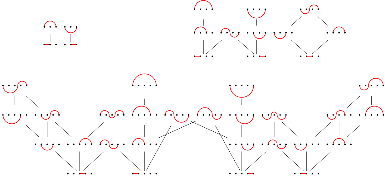
FIGURE 7. The weak orders of size 3 (top left), 4 (top right), and 5 (bottom) restricted to their join irreducibles represented by the corresponding arcs.
