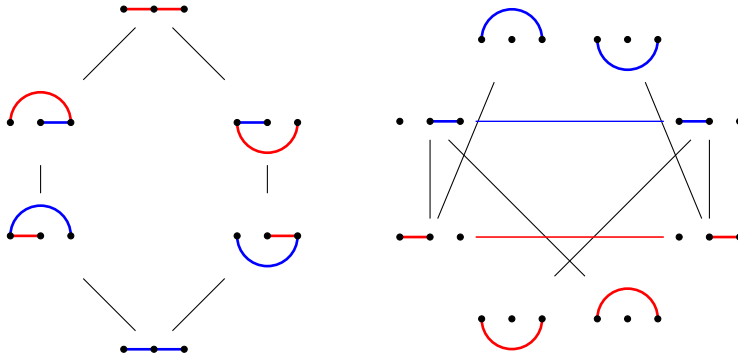
FIGURE 9. The weak order on \mathfrak{S}_3 with permutations labeled by semi-crossing arc bidiagrams, and the canonical complex of \mathfrak{S}_3 with join and meet irreducible permutations labeled by arcs.
