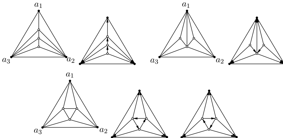
Figure 3: Three triangulations and their 3-orientations.
