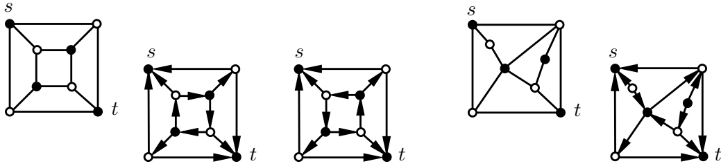
Figure 1: Two quadrangulations and their 2-orientations.
