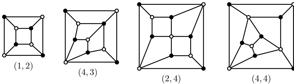
Figure 2: All prime quadrangulations with 5, 7 and 8 inner faces. A pair (a, b) below a quadrangulation Q indicates that Q allows a non-isomorphic choices of s, t on the outer face and it has b 2-orientations for each choice. This yields p_5 = 2 , p_7 = 12 and p_8 = 24 .
