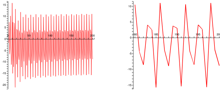
Figure 1: Permutations with distinct cycle lengths: the approximation error as measured by n^3(f_n/\widehat{f}_n^{[1]} - 1) , with \widehat{f}_n^{[1]} truncated after n^{-3} terms, for n = 1..200 (left) and for n = 180..200 (right).
