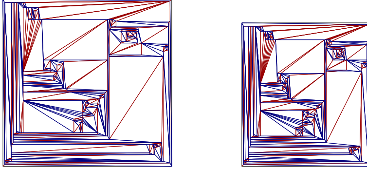
Fig. 12. A random triangulation with 200 vertices embedded with the algorithms DRAW and COMPACTDRAW.
