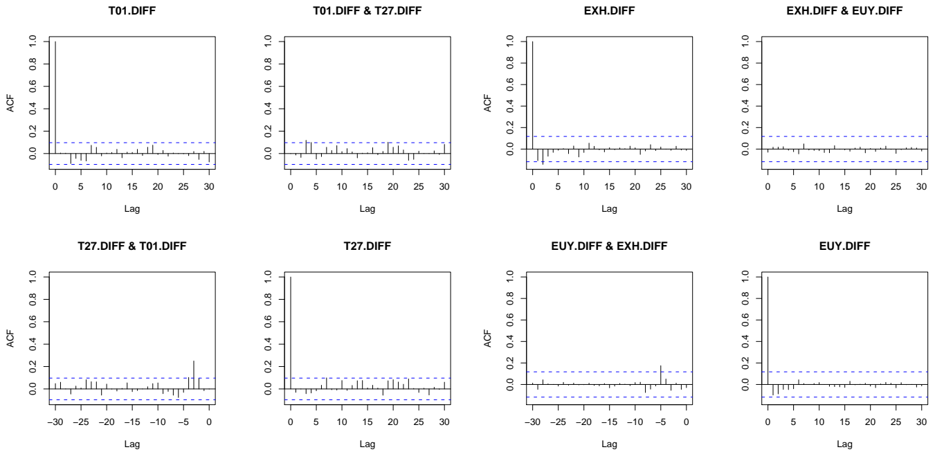
Figure 4. Cross-correlation matrices. Left: local neighbors. Right: non-local sectors
