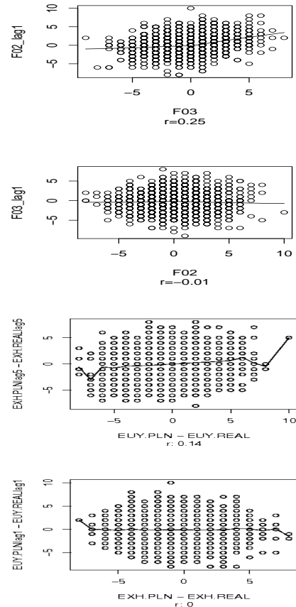
Figure 6. Scatterplots of gaps in one sector against time-lagged gaps in other sectors. First and third panel: significant coefficients (Japan/Europe), second and fourth: non-significant coefficients.
