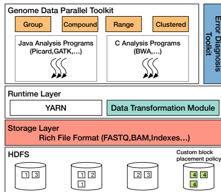
Figure 2: Gesall Architecture. The diagram illustrates the architecture of the Gesall platform. It is divided into several layers: the Genome Data Parallel Toolkit (containing Java and C analysis programs), the Runtime Layer (with YARN and a Data Transformation Module), the Storage Layer (using Rich File Format like FASTQ, BAM, and Indexes), and HDFS (with a Custom block placement policy). The Error Diagnosis Toolkit is shown as a vertical component on the right.
