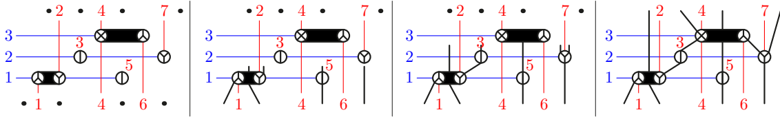
FIGURE 24. The insertion algorithm on the decorated ordered partition \underline{1}25|37|\underline{4}6 .
