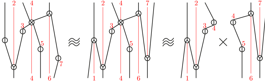
FIGURE 4. Some bijections between permutrees: the leftmost and rightmost decorations do not matter (left), and a decoration \otimes yields a product (right).
