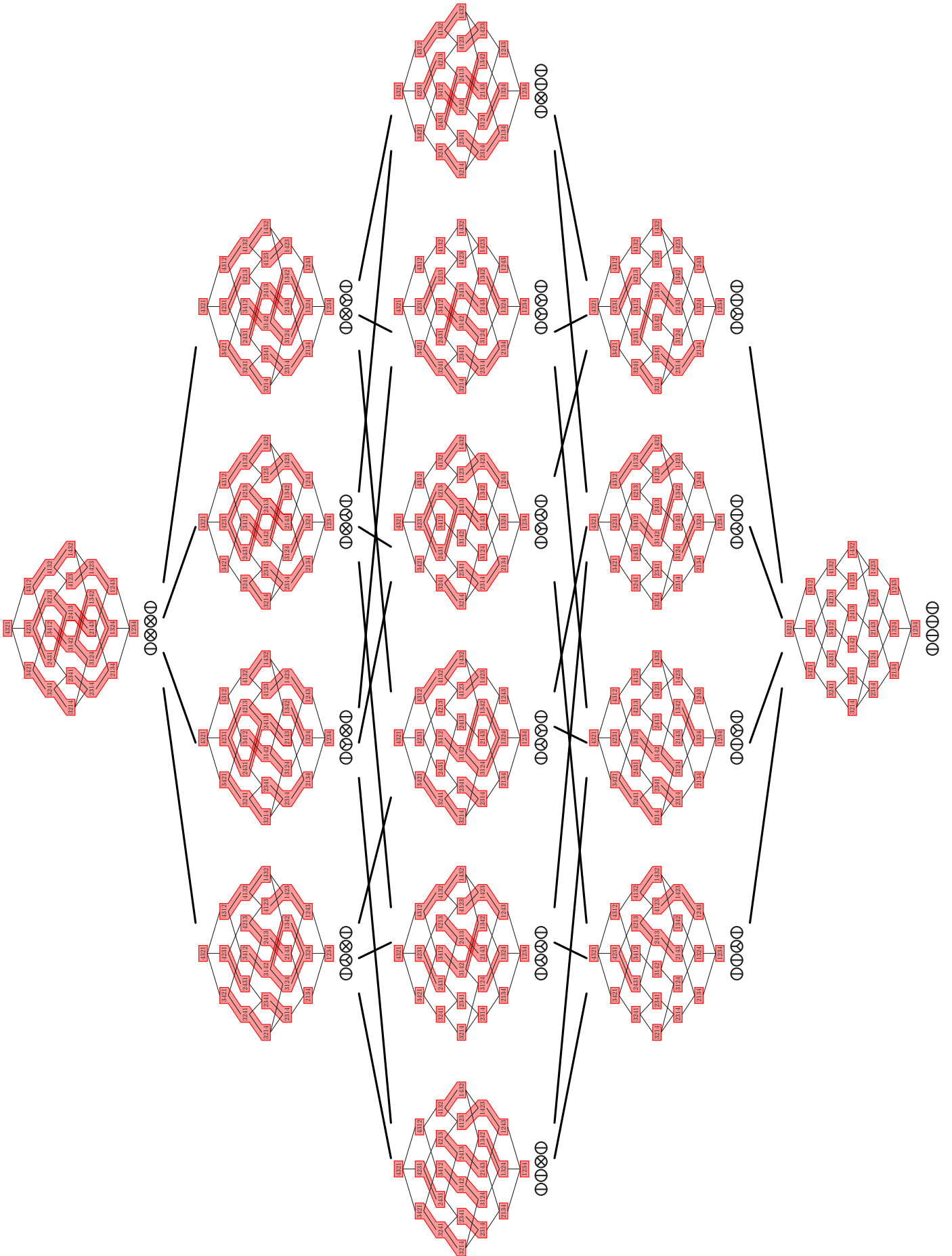
FIGURE 14. The fibers of the \delta -permutree congruence, for all decorations \delta \in O \cdot \{O, O, O, O\}^2 \cdot O .
