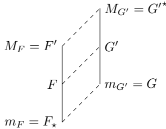
FIGURE 12. Meet-semidistributivity in the facial weak order.
