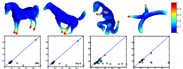
Figure 3. HKS function and its persistence diagrams.
