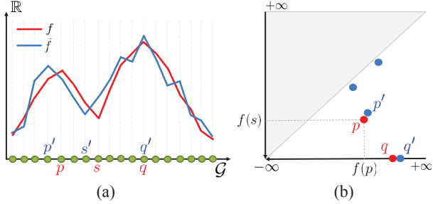
Figure 2. Sketch of persistence computing: (a) a smooth function f maps the nodes of \mathcal{G} to \mathbb{R} , \hat{f} is a noisy version of f ; (b) superimposition of PDs of f (red) and \hat{f} (blue), showing the one-to-one correspondence between the prominent peaks of f and \hat{f} .
