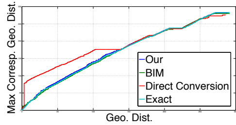
(a) Maximal distortion computed with Eq. (10)
