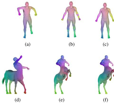
Figure 6: Visualization of the point-to-point mapping through color correspondence. The texture of the first column (6a, 6d) are transferred to the second using the direct conversion of a functional map (6b, 6e) and to the third using our method (6c, 6f).
