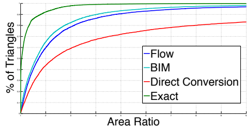
(b) Area ratio
