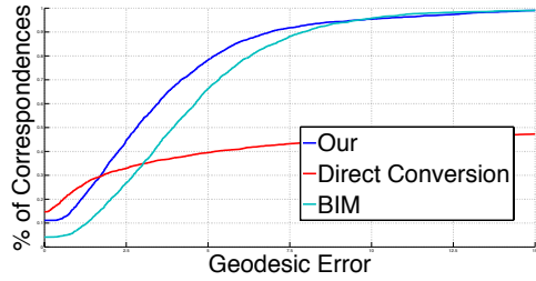
(b) TOSCA: average from 5 pairs
