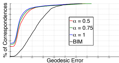
Figure 3: Impact of the noisy functional map C_T^\alpha on the point-to-point correspondences for various values of \alpha .
