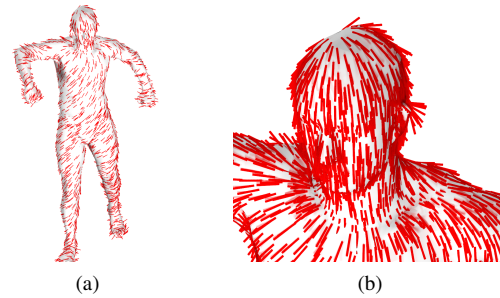
Figure 8: Visualization of the direction of the optimal vector field corresponding to the experiment 7c: complete shape 8a and close-up on the face 8b.
