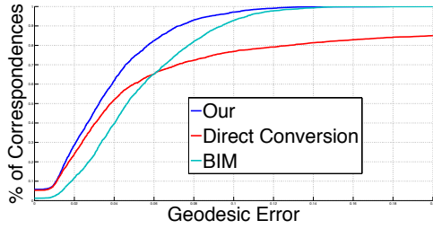
(a) SCAPE: average from 7 pairs
