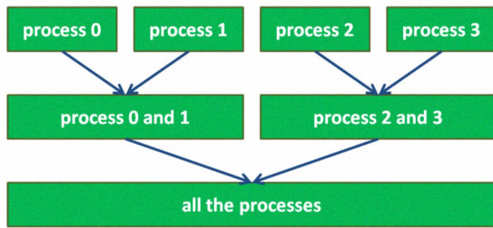
Fig. 1. The classic communication schema “cascade”, where only \log_2 p communication phases are needed to the processes for sharing an information.
